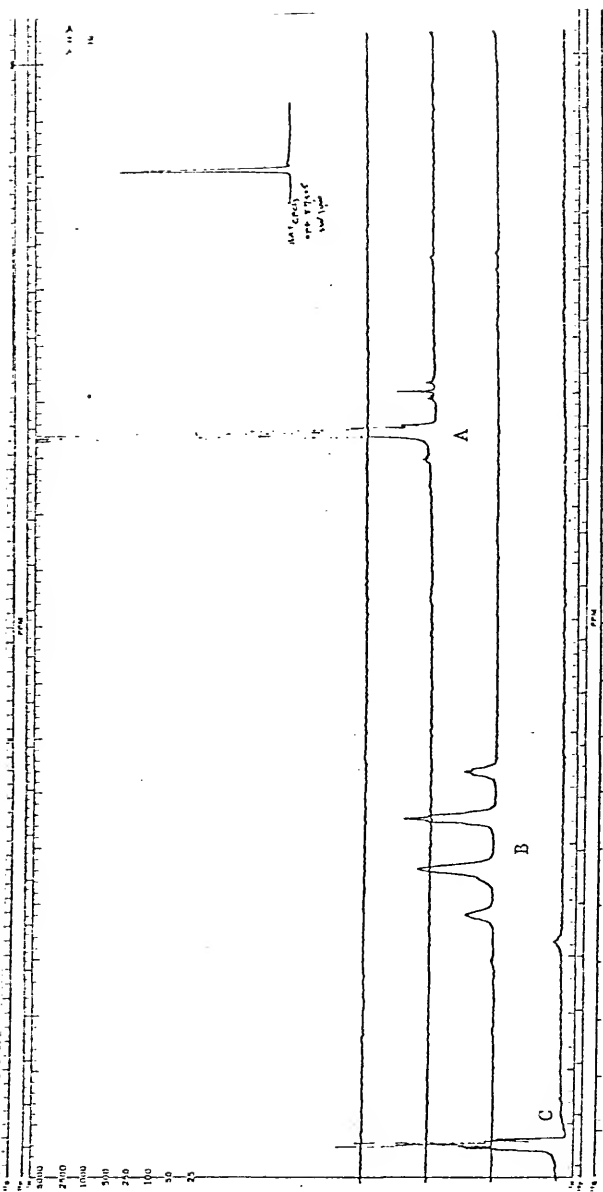
Figure 49 - 19 F NMR of \text{CF}_2\text{CF}=\text{CHCH}(\text{CH}_3)_2
